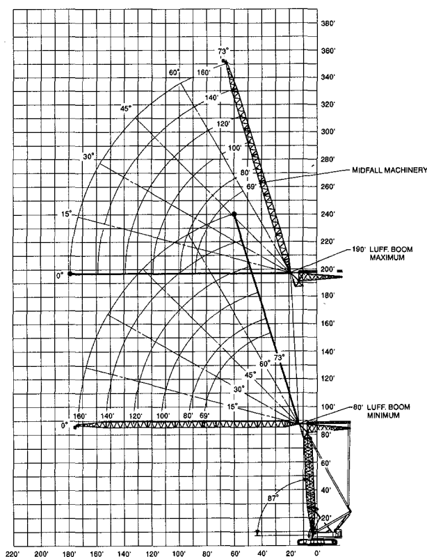
Operating Radius
