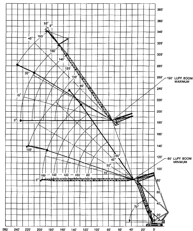
Operating Radius
